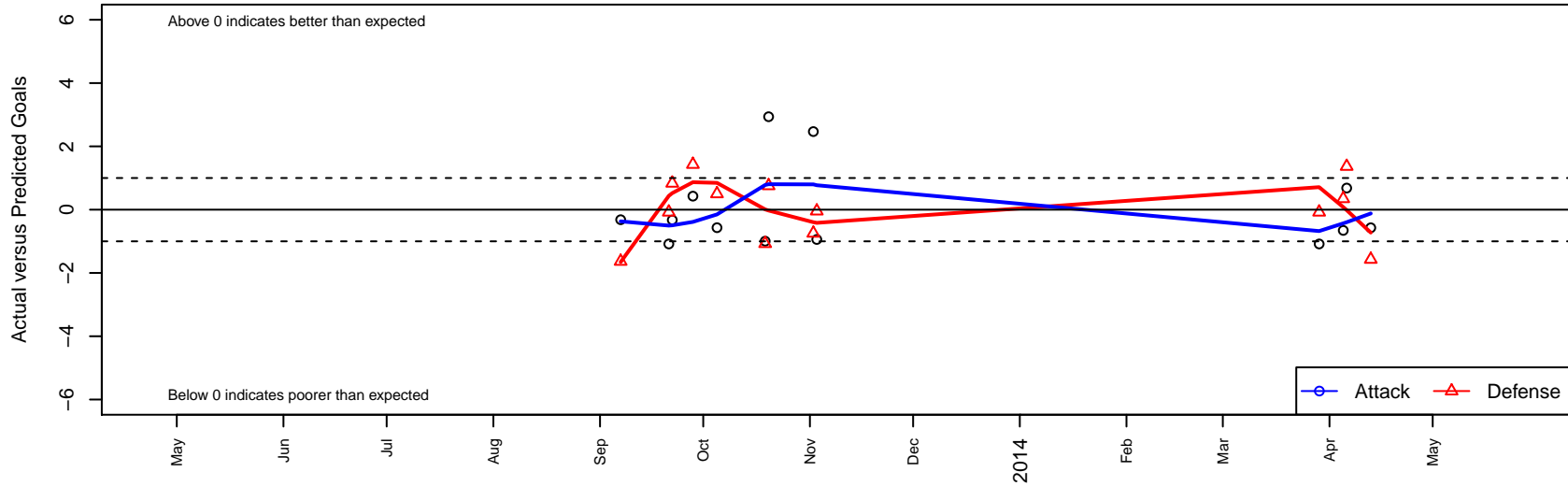
Internationals SC ECNL G99 Dots are actual minus expected GF (blue circles) and GA (red triangles). Blue line is smoothed change in attack strength. Red is smoothed change in defense strength.
